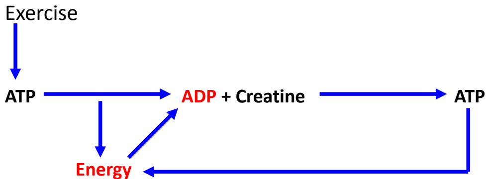
A simplified illustration of how creatine works to re-generate ATP from ADP.
